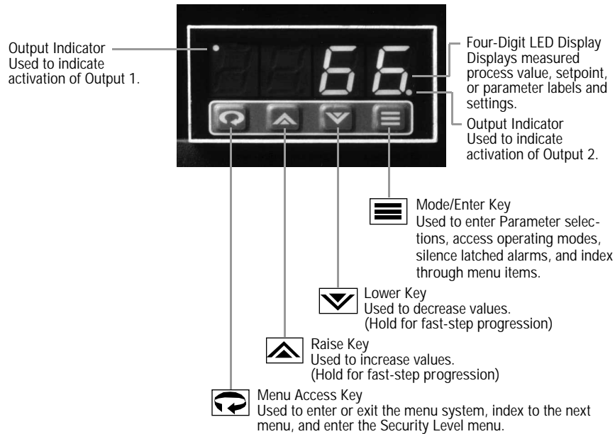
Figure 8. Front Panel Controls and Indicators
