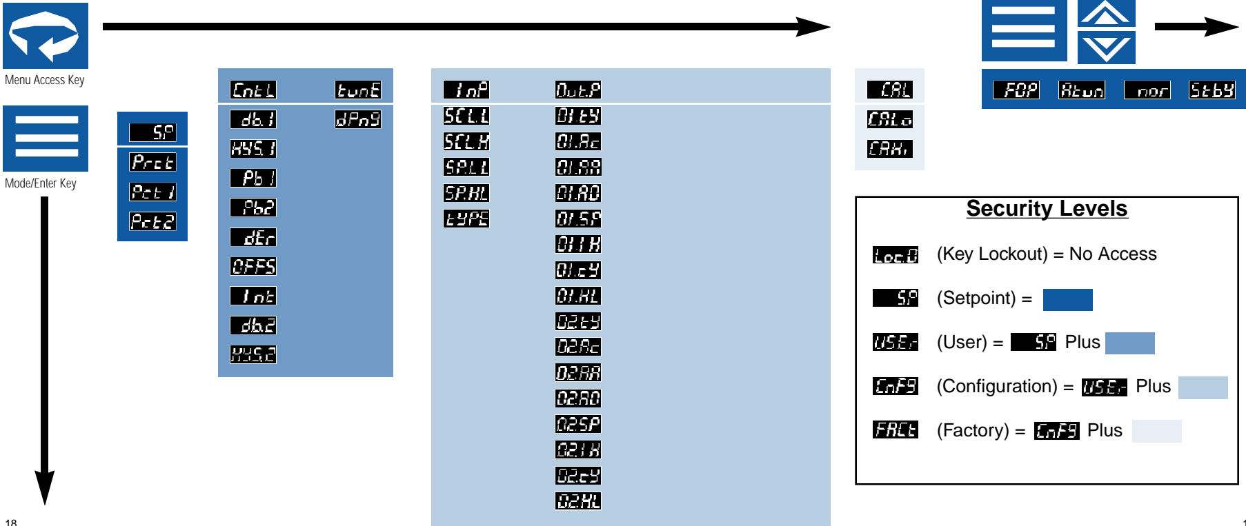
Figure 10. Overview of Series 32C Menu System, Operating Modes, and Security Levels
