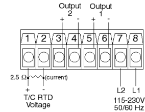
Figure 4. Contact Identification
