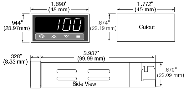
Figure 2. Case Dimensions
