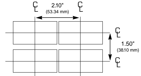
Figure 1. Recommended Panel Layout for Multiple Controllers
